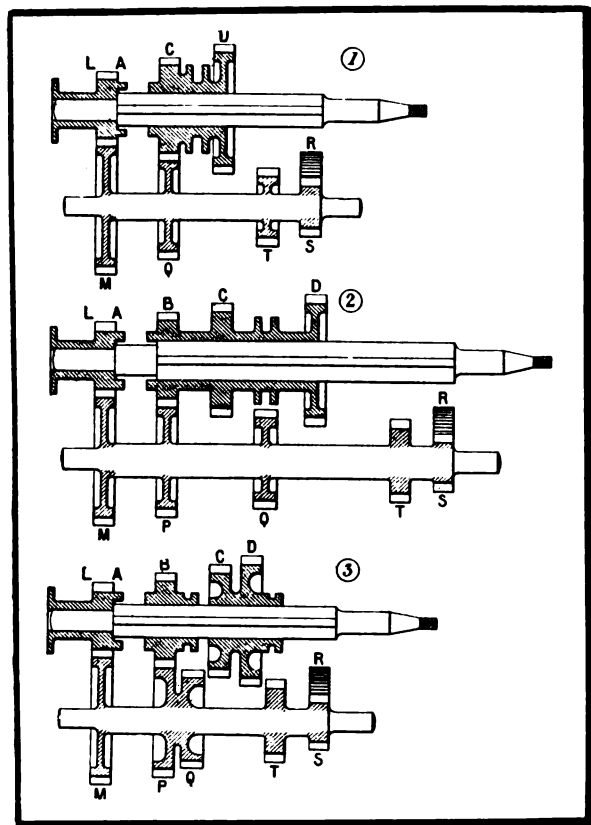
Fig. 1.—Types of change gears: No. 1, three speeds. N. 2, four speeds, one sliding member. No. 3, four speeds, two sliding members.
